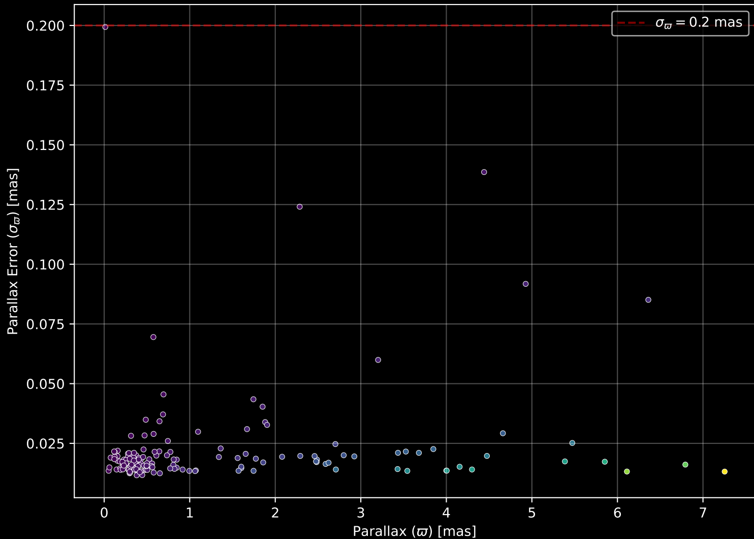
APOGEE DR17 Field: [240+18] Parallax Quality (n= 154)
