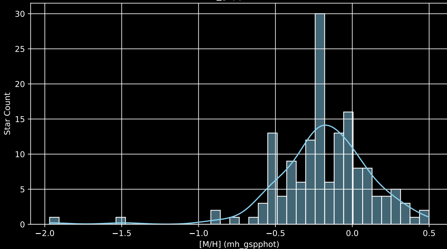
APOGEE DR17 Field: [240+18 [M/H] (mh_gspphot) (n= 153)
