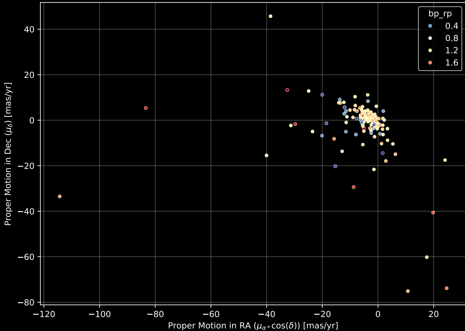
APOGEE DR17 Field: [240+18] Proper Motion Diagram (n= 154)
