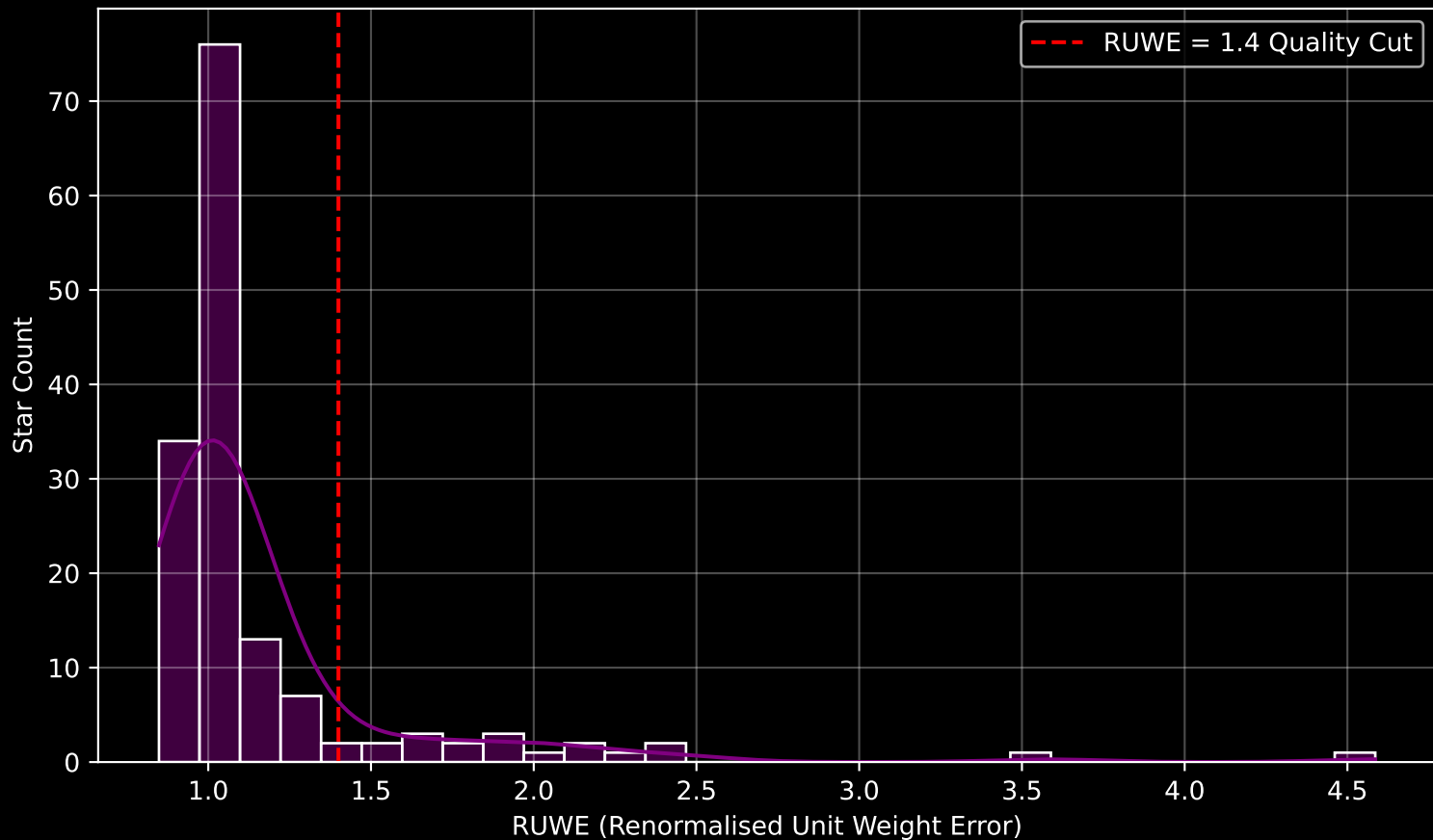
GAPOGEE DR17 Field [240+18] RUWE Distribution (n= 150)
