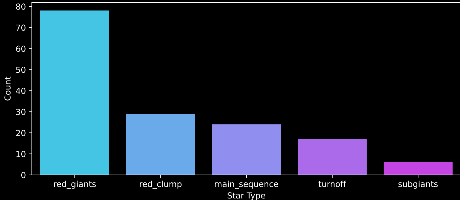
APOGEE DR17 Field: [240+18] Count plot of Star Type
